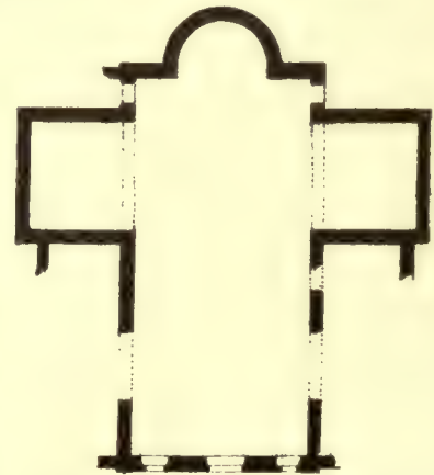
Fig. 42.—Como. Plan of the ancient Basilica of SS. Peter and Paul, now Sant' Abondio (Vth Century). (From Boito, "Architettura del medio evo in Italia.")
